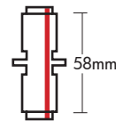
Coupler T433D
